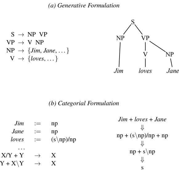
Figure 2. (a) A very simple Chomskian grammar and the parse tree for “Jim loves Jane”, as compared with (b) a categorial equivalent, including the combination rules, and its derivation. Note the clear structural relationships between the two, but also that (a) has the implication of parsing from top to bottom, while (b) is explicitly parses up, from the words, and discovers a sentence. Abbreviations: n is noun, v is verb, p is phrase; X and Y are variables.
